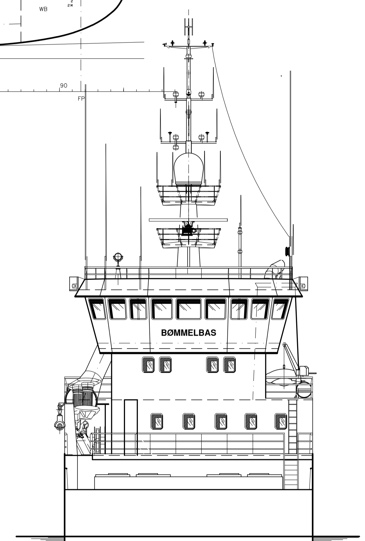
SECTION IN FRONT OF WHEELHOUSE
